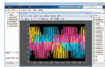
MATLAB *
